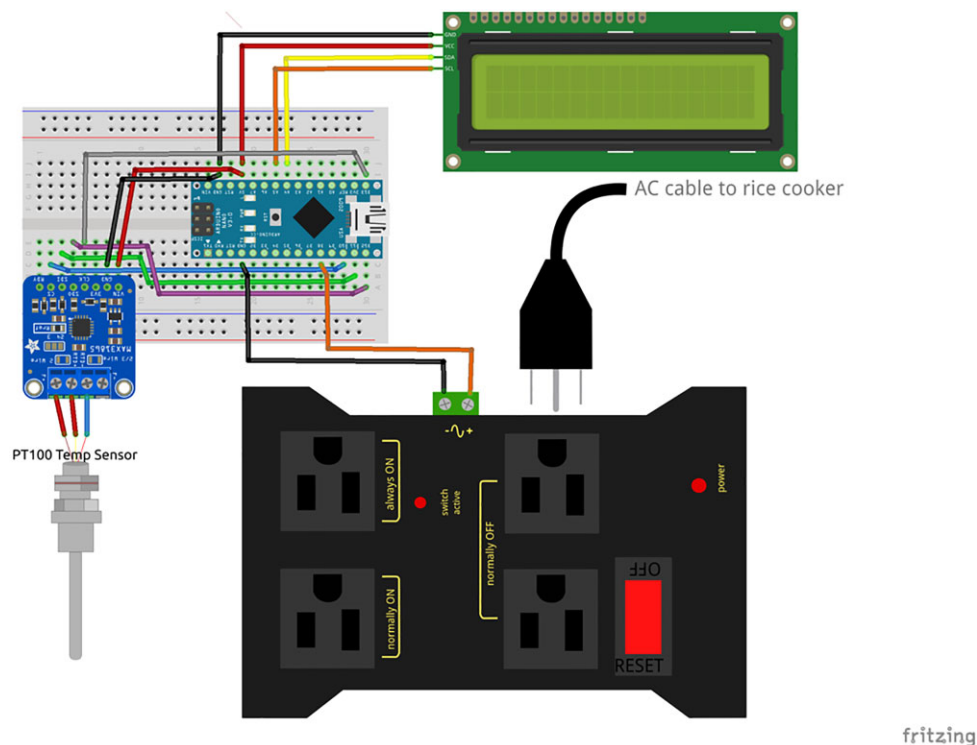
Fig. 1 Fritzing diagram of rice cooker.
